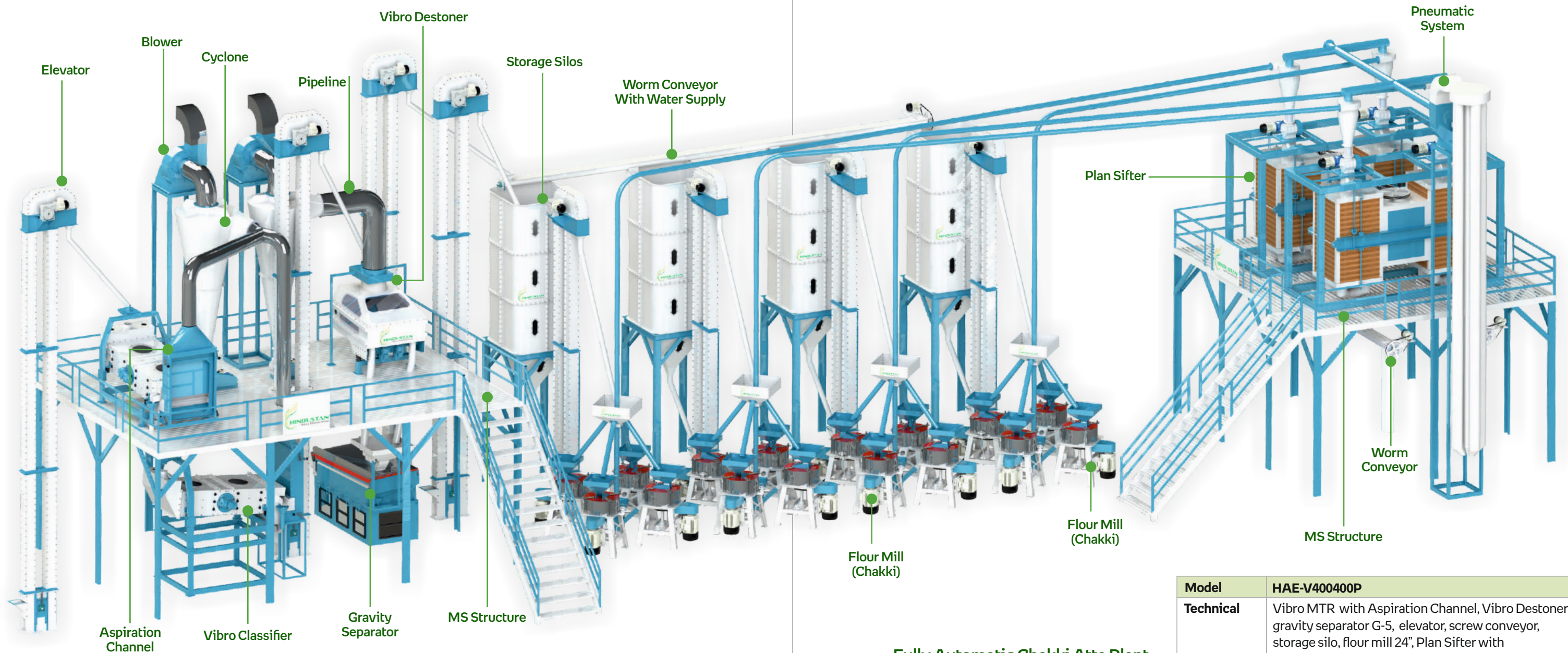
Fully Automatic Chakki Atta Plant with Multipurpose Vibro Cleaning
